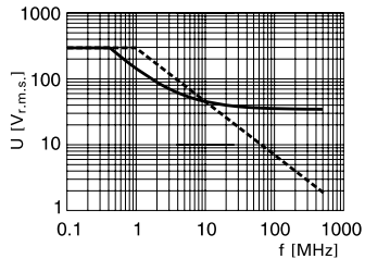
Isoprobe IV
